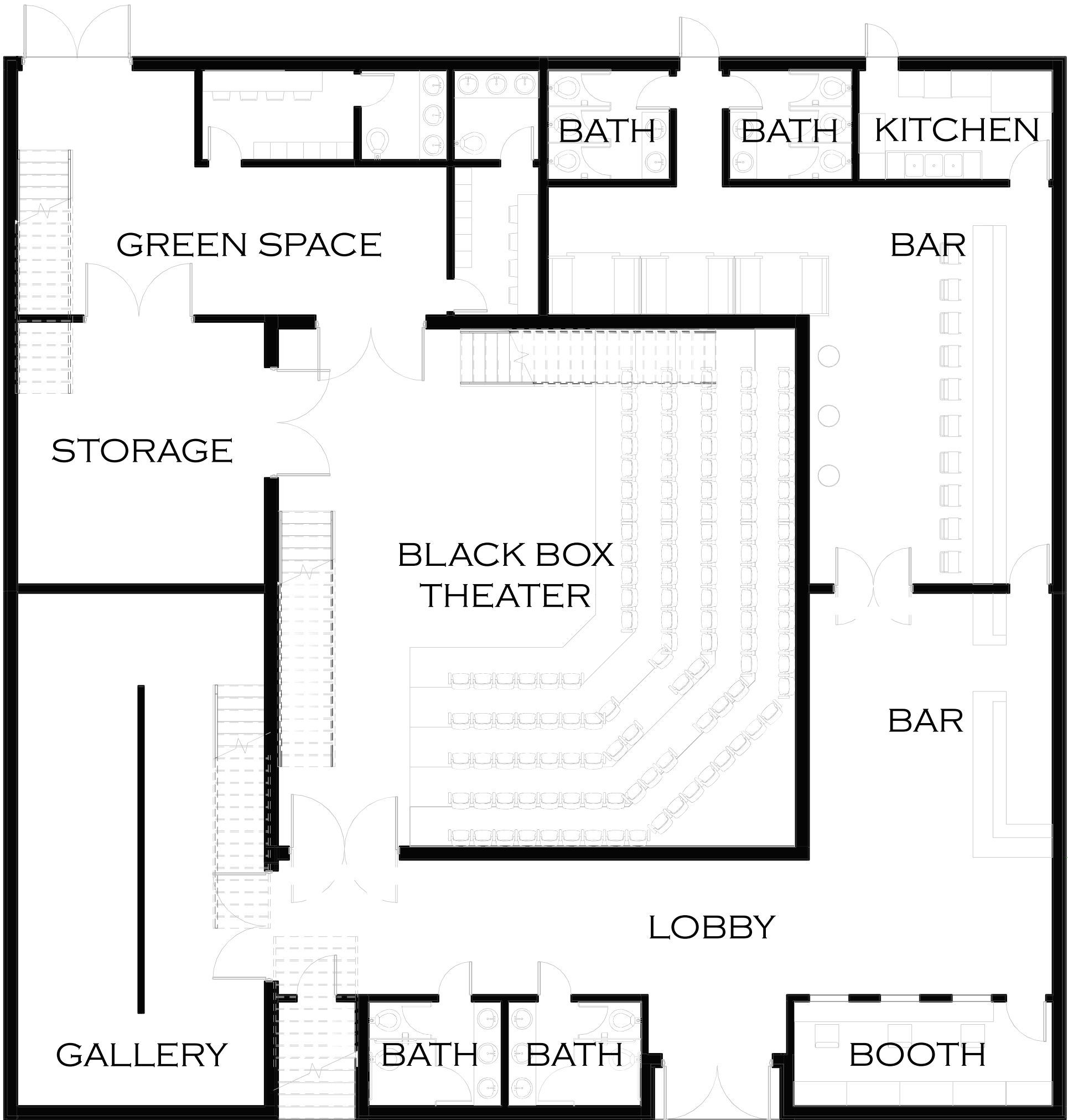
FIRST FLOOR
