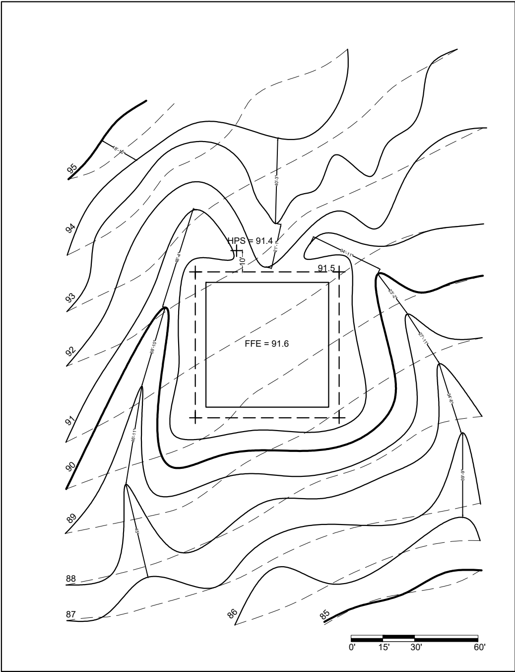
1 SWALE W/ CONCRETE SLAB SCALE: 1" = 30'
