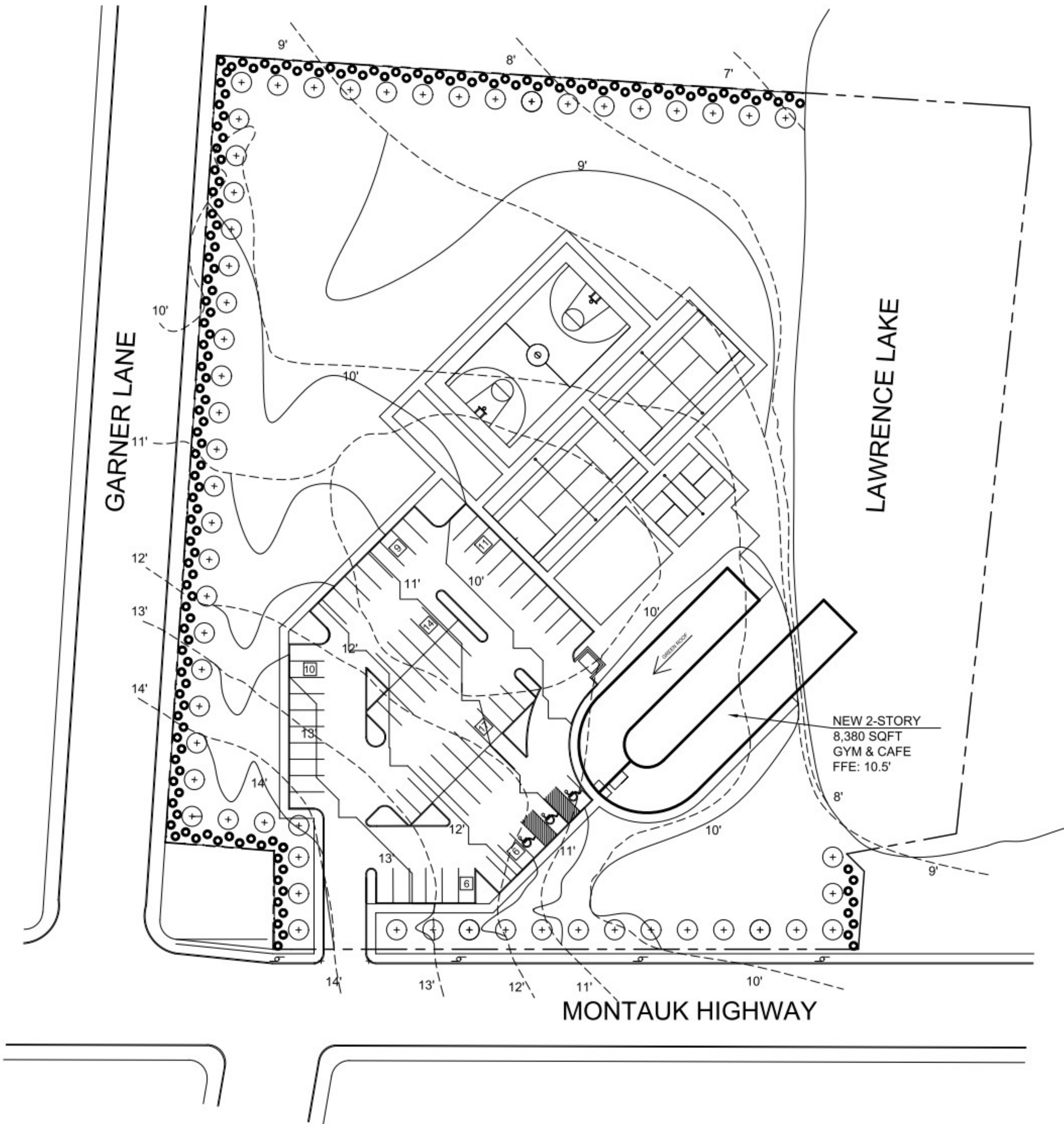
2 PROPOSED SITE PLAN 1" = 40'-0"
