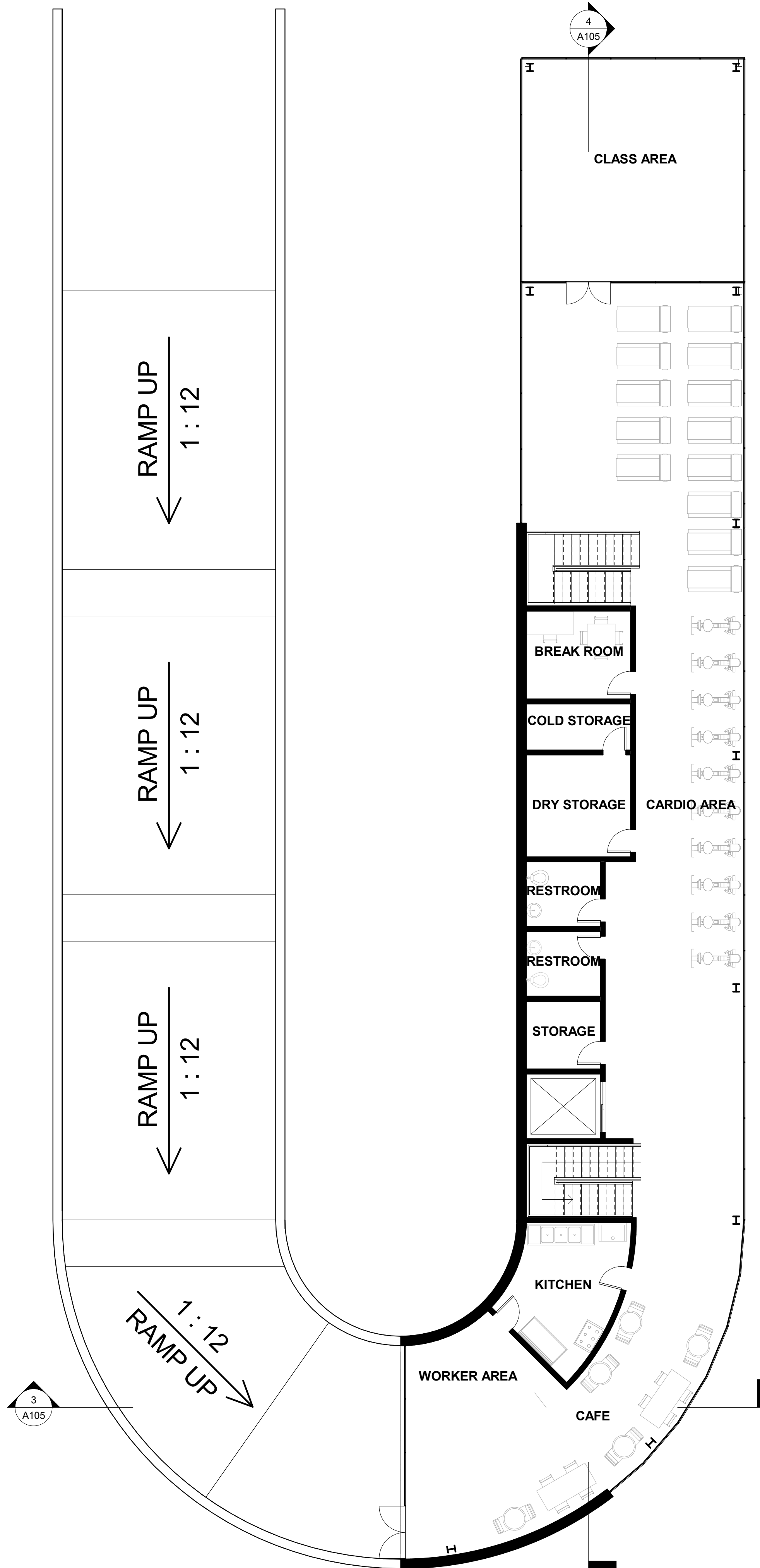
① SECOND FLOOR PLAN 1/8" = 1'-0"
