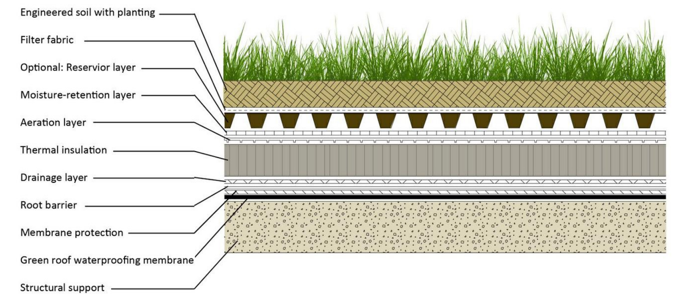
TYPICAL GREENROOF DETAIL
